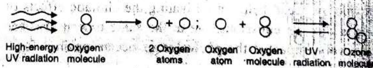
Fig. Schematic representation of the formation of stratospheric ozone
